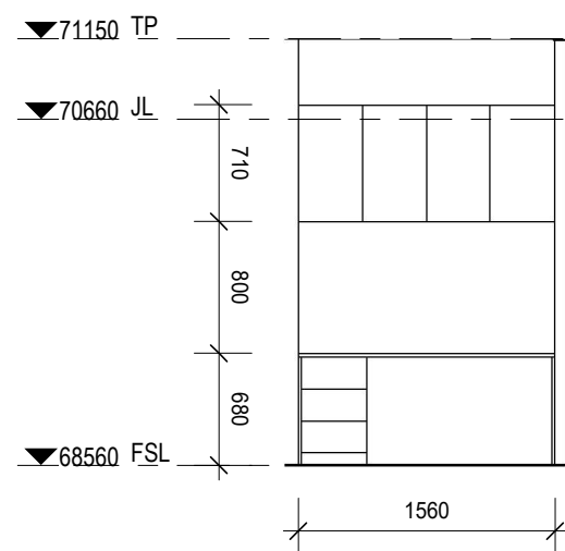
STUDY NOOK ELEVATION 1 : 50
