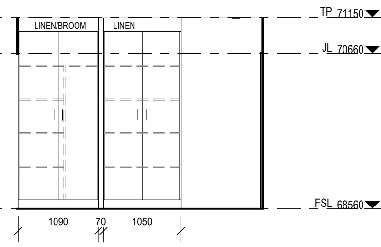
LAUNDRY ELEVATION 2 1 : 50
