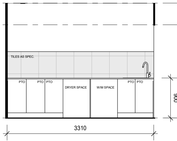
LAUNDRY ELEVATION 1 1 : 50
