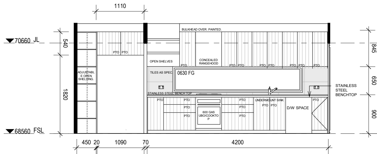
KITCHEN/PANTRY ELEVATION 1 1 : 50
