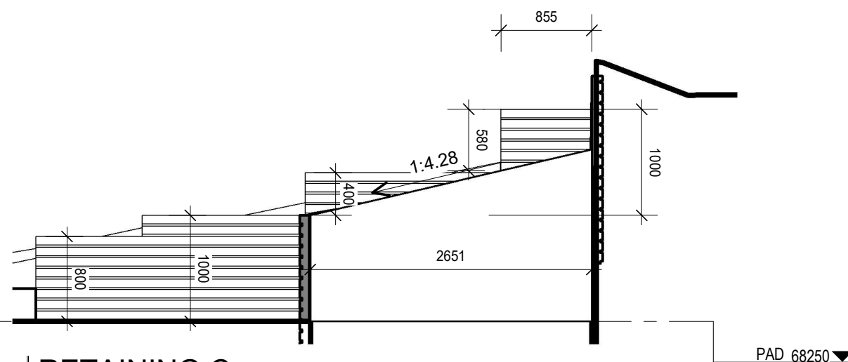
RETAINING C
