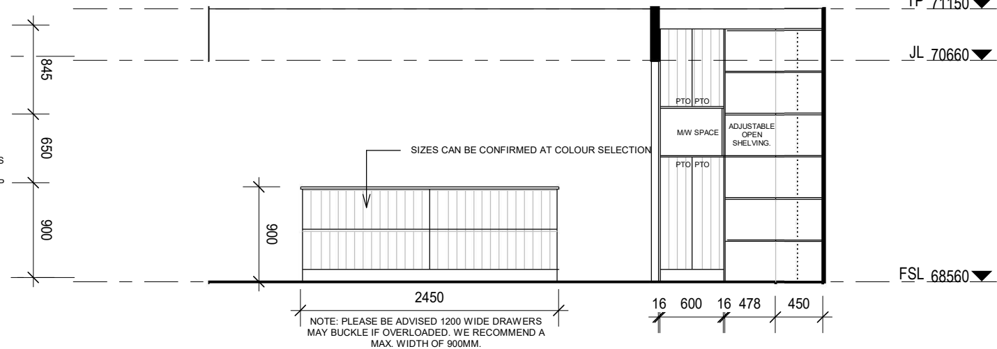
KITCHEN/PANTRY ELEVATION 2 1 : 50
