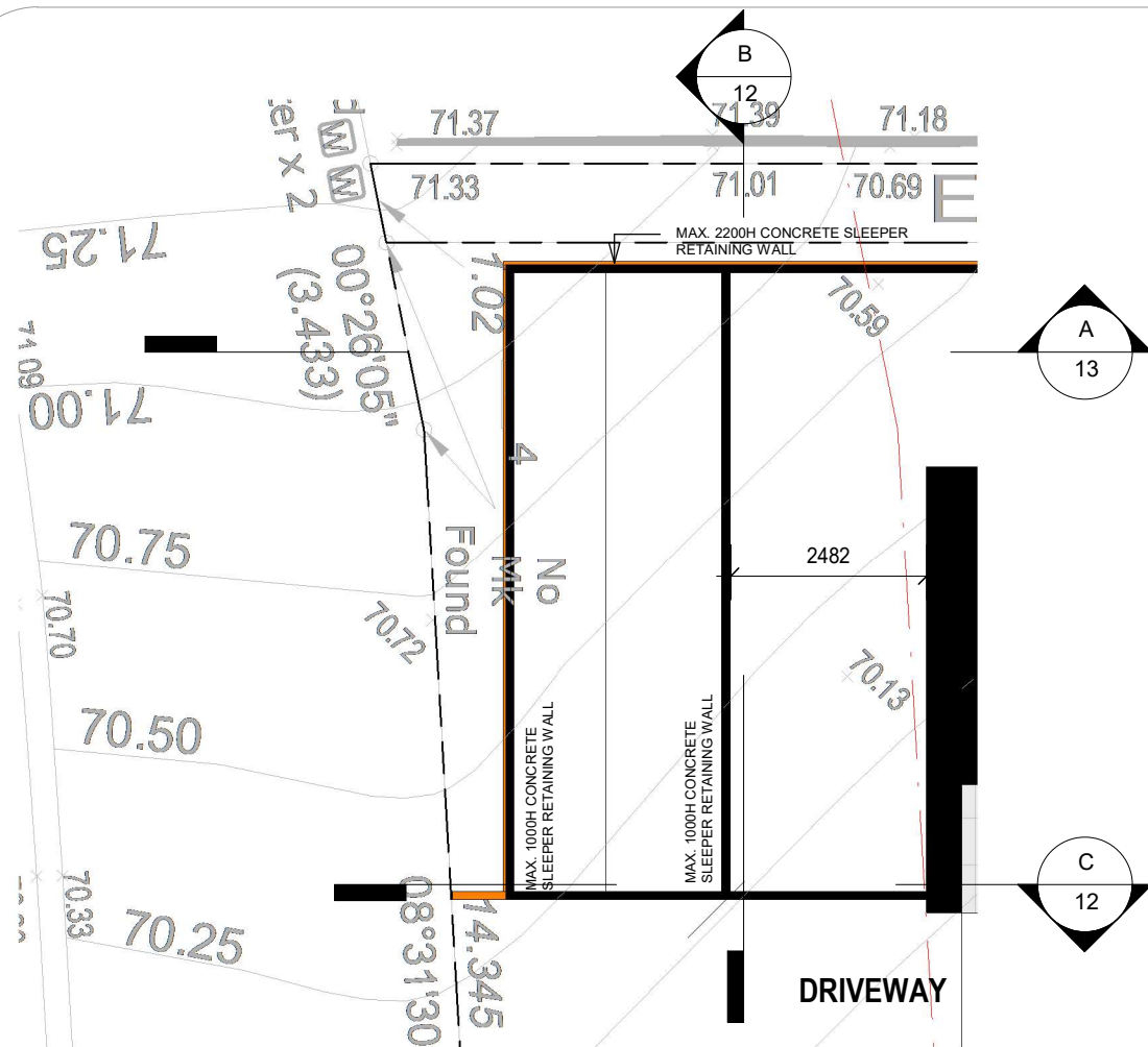
RETAINING PLAN
